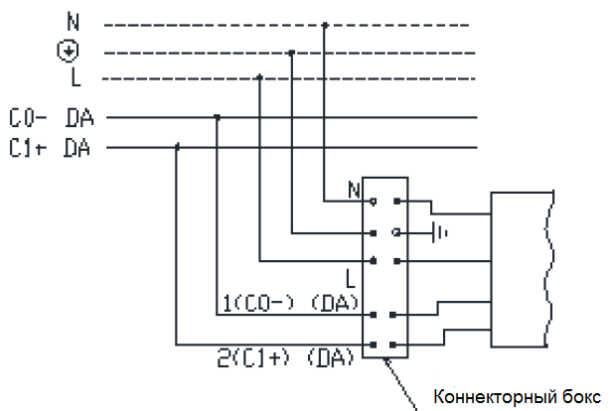
Terminal block
