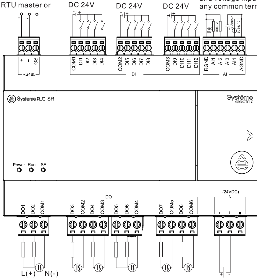
External 24VDC power input
