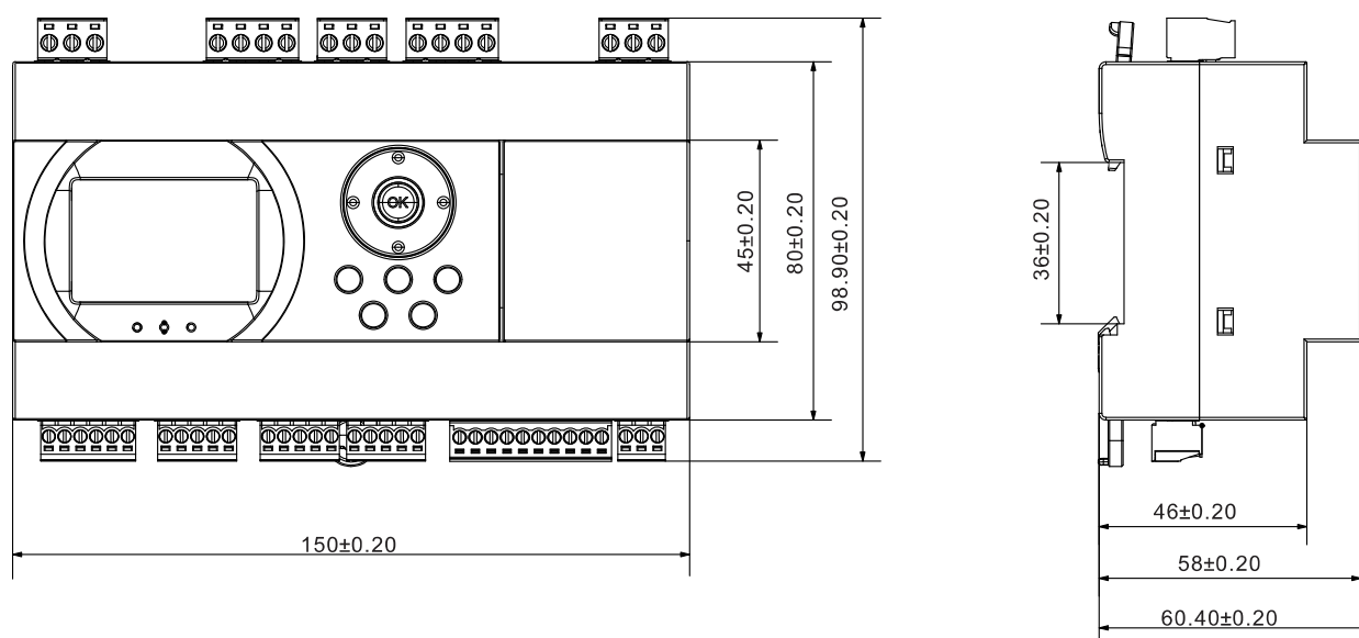
Figure 2-1 Smart Relay Series Controller Dimensions (mm)
