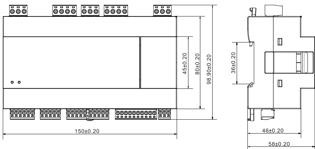
Figure 2-2 SM172EMIO2800 Hybrid Module Dimensions (mm)
