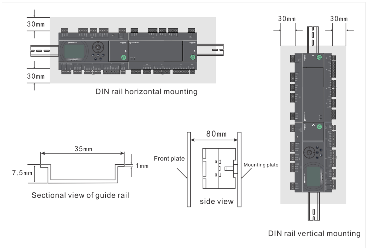
Figure 2-3 Installation Diagram
