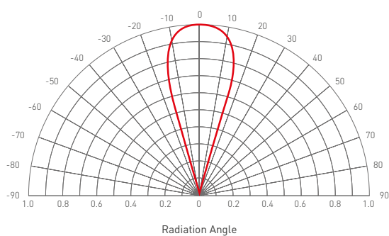
Radiation Characteristics
