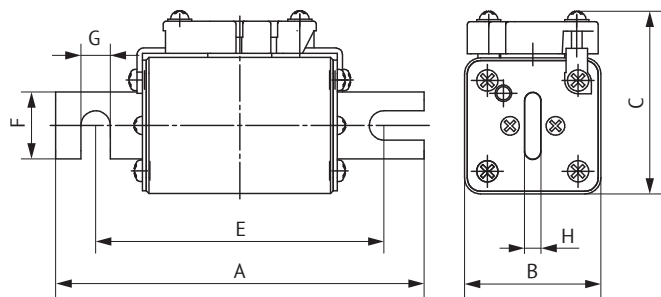
OptiFuse FR S70, S71, S72, S73. D11 connection type
