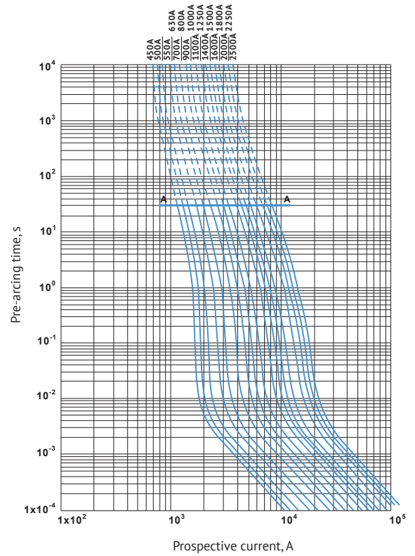
CTC of both full disconnection and fusing for S33 size
