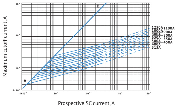
Cutoff current amplitudes versus prospective SC current for S32 size
