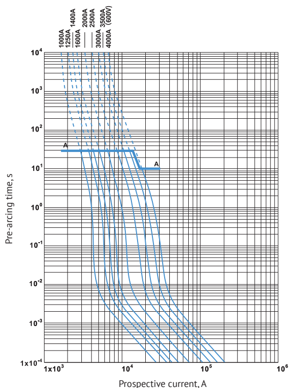
CTC of both full disconnection and fusing for S44 size
