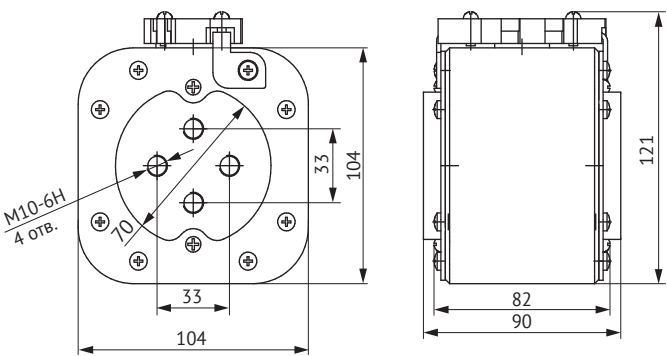
OptiFuse FR S84. TF connection type
