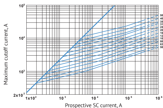
Cutoff current amplitudes versus prospective SC current for S70 size
