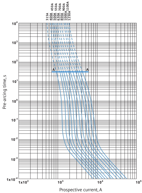
CTC of both full disconnection and fusing for S32 size
