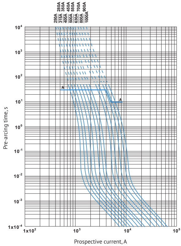
CTC of both full disconnection and fusing for S72 size
