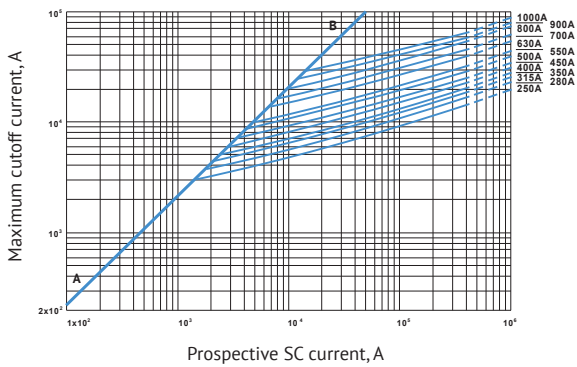
Cutoff current amplitudes versus prospective SC current for S72 size
