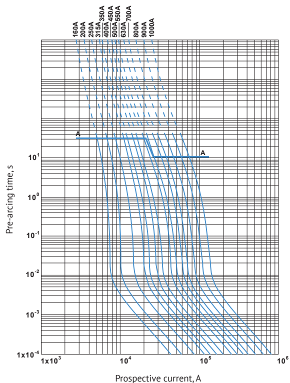
CTC of both full disconnection and fusing for S71 size
