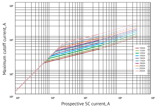
Cutoff current amplitudes versus prospective SC current for S44 size
