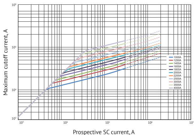
Cutoff current amplitudes versus prospective SC current for S44 size
