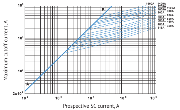
Cutoff current amplitudes versus prospective SC current for S73 size
