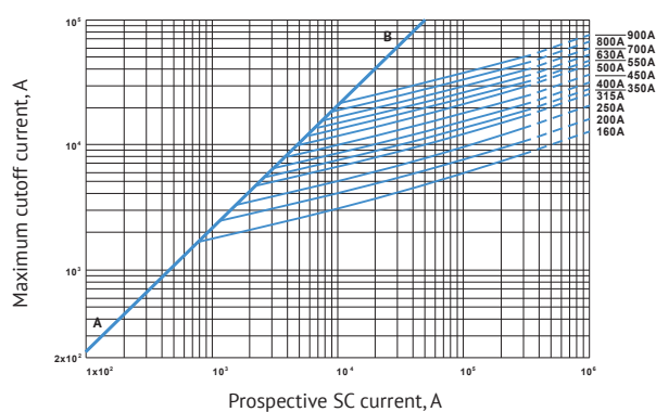
Cutoff current amplitudes versus prospective SC current for S71 size
