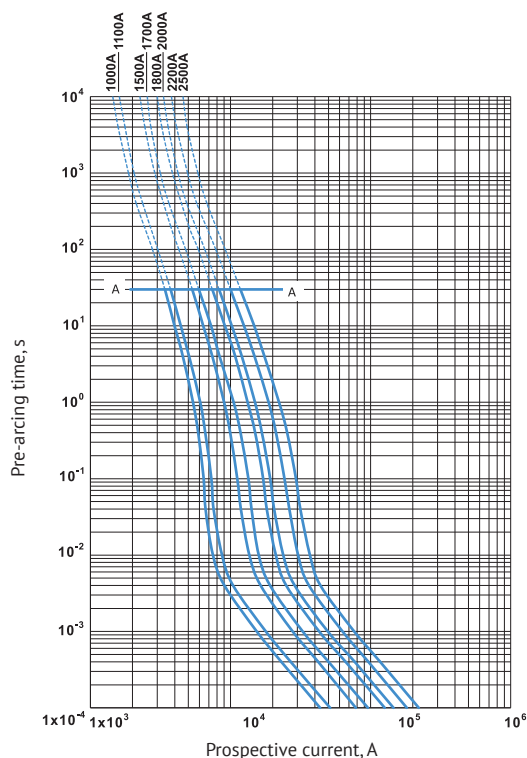
CTC of both full disconnection and fusing for S84 size
