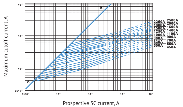
Cutoff current amplitudes versus prospective SC current for S33 size
