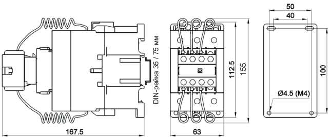
MC1DPK, MC1DTK
