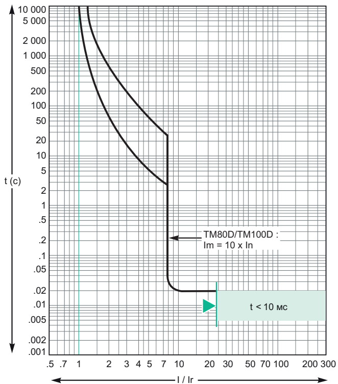
TM80D/TM100D
