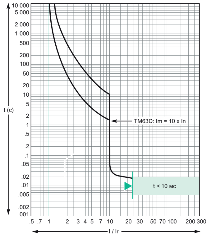
TM63D
