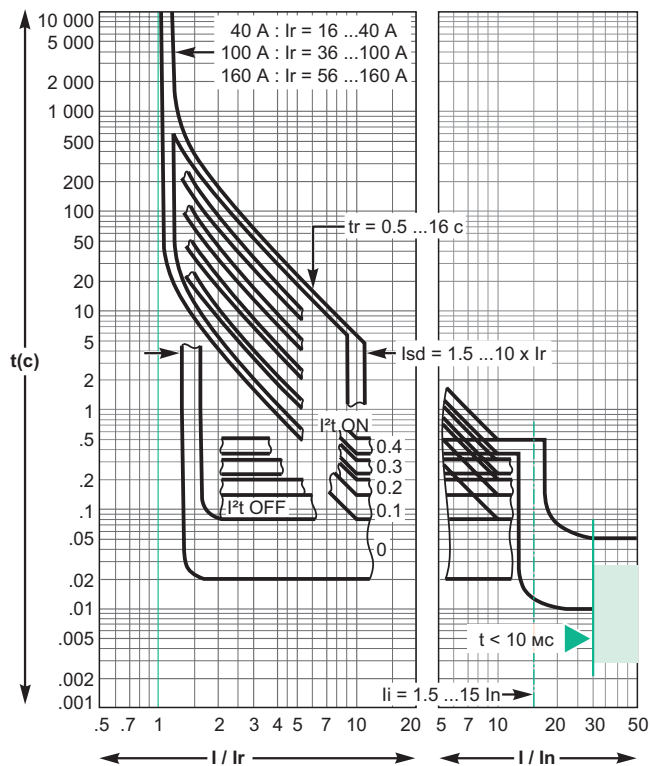
SystemeLogic 5.2E 40...160
