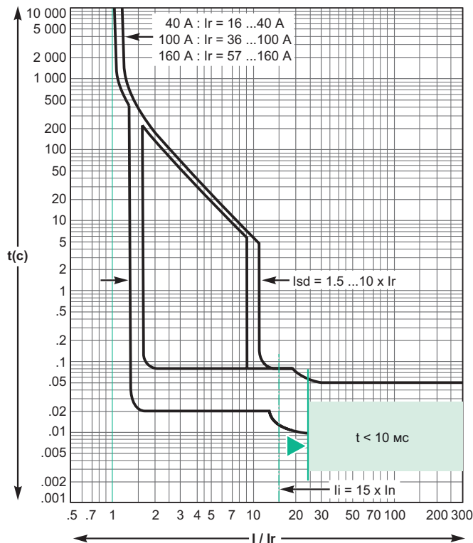
SystemeLogic 2.2 40...160
