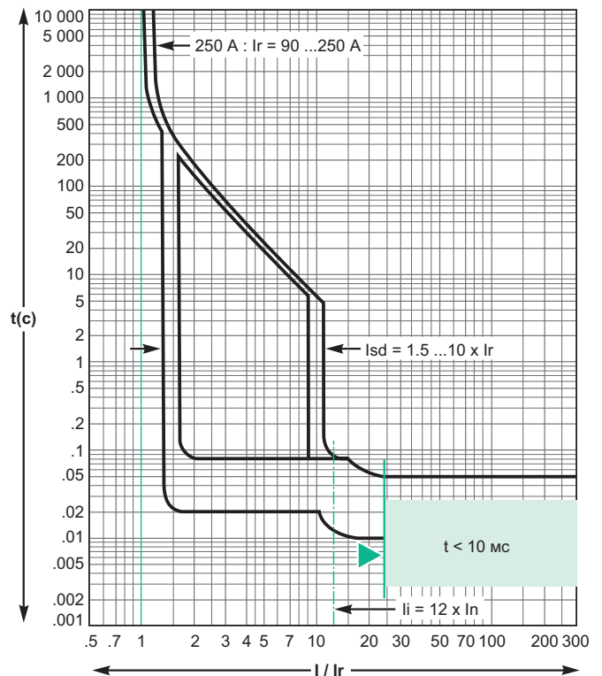
SystemeLogic 2.250
