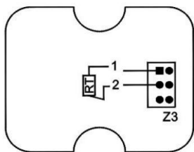
NTC10K
