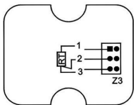
PT1000
