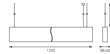
PROFILE 30 H 1250
